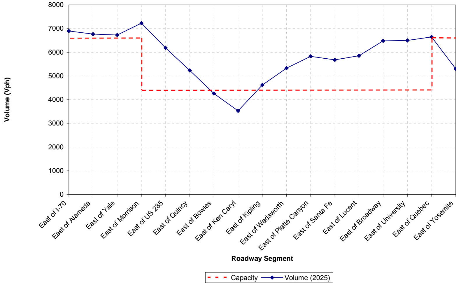
Figure 8.3 V/C Comparison - Projected (2025)
